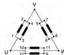
Delta parallel connection 115 V - 50 Hz 138 V - 60 Hz
