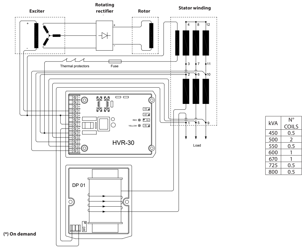
Fig. 19 - CONNECTING THE DP01 WITH REGULATOR HVR-30 WITH VOLTAGE REFERENCE THREE-PHASE (PRO 35)
