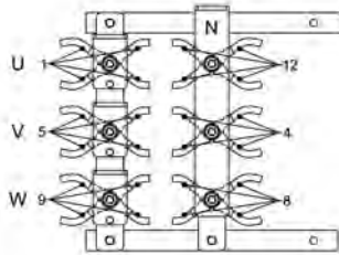
Star connection + neutral 230/400 V - 50 Hz 276/480 V - 60 Hz
