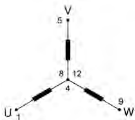
Star connection+neutral
