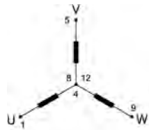
Star connection + neutral 230/400 V - 50 Hz 276/480 V - 60 Hz
