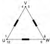
Delta connection 230 V - 50 Hz 276 V - 60 Hz
