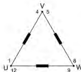
Delta connection
