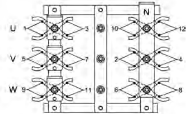
Star connection parallel+ neutral 200/115 V - 50 Hz 240/138 V - 60 Hz
