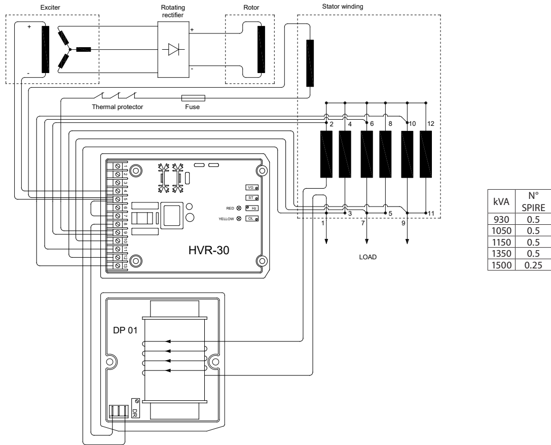
Fig. 20 - CONNECTING THE DP01 WITH REGULATOR HVR-30 WITH VOLTAGE REFERENCE THREE-PHASE (PRO 40)
