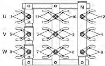
Star connection serie+ neutral 230/400 V - 50 Hz 276/480 V - 60 Hz
