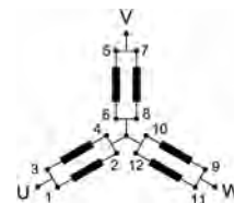
Star connection parallel+ neutral 200/115 V - 50 Hz 240/138 V - 60 Hz
