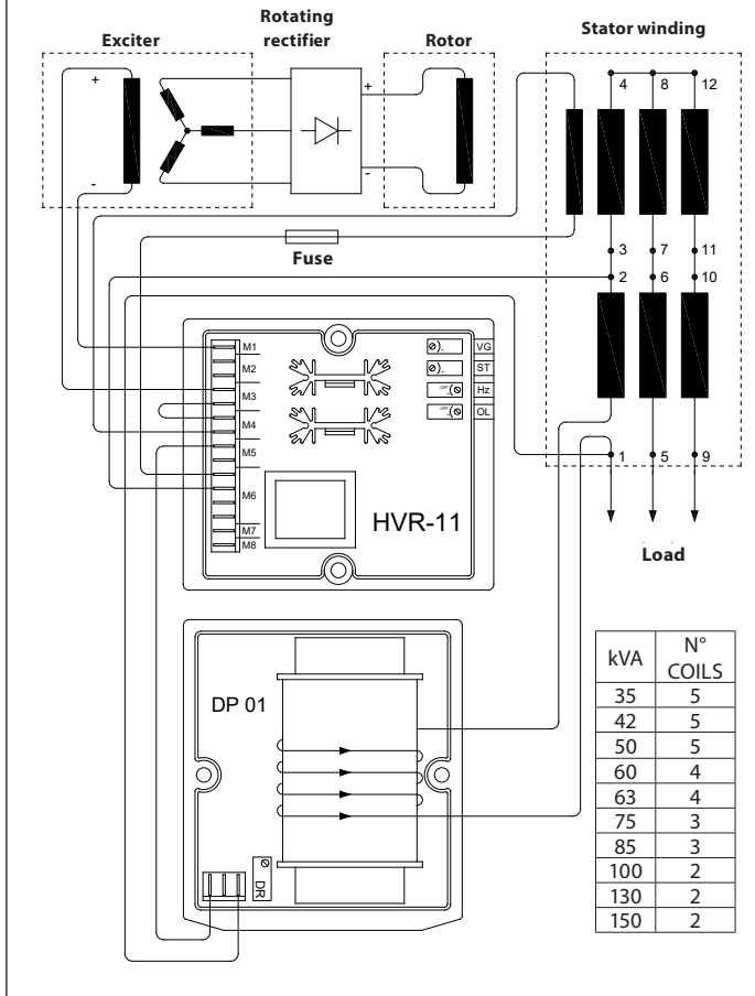
Fig. 17 - CONNECTING THE DP01 WITH REGULATOR HVR-11
