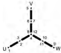
Star connection serie+ neutral 230/400 V - 50 Hz 276/480 V - 60 Hz
